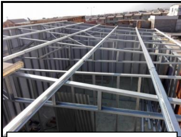
The frame of the 2nd story roof
